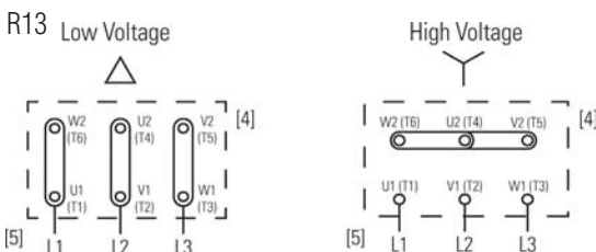
Motor Connection Diagrams (Above)
